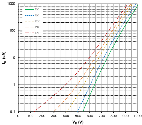
Figure 3. Reverse Characteristics
