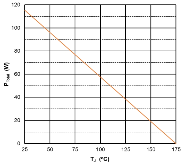
Figure 4. Power Derating
