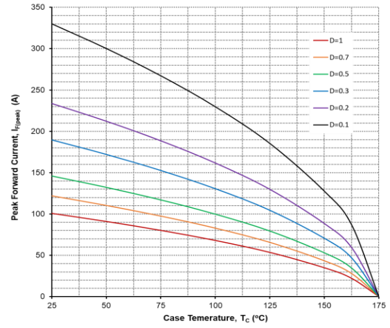
Figure 8. Current Derating
