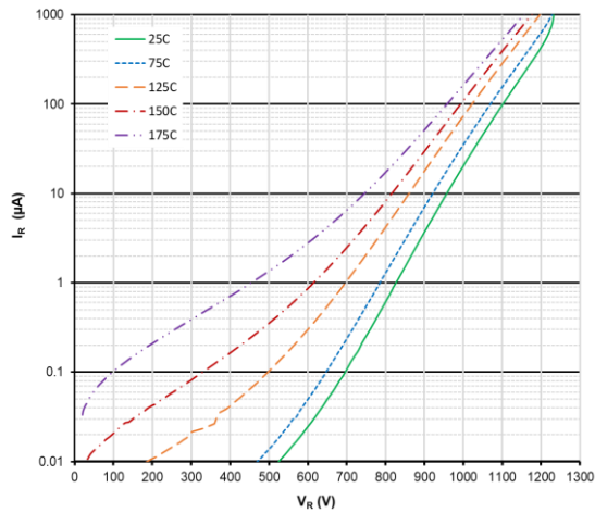
Figure 3. Reverse Characteristics
