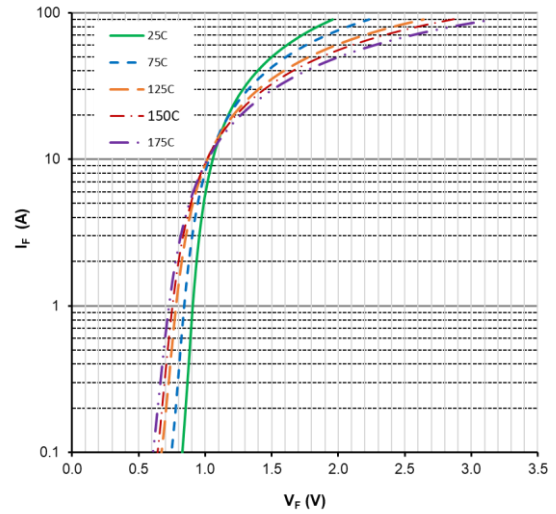
Figure 2. Forward Characteristics
