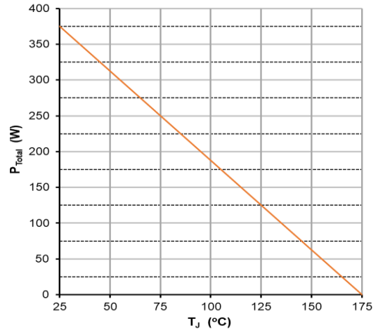
Figure 4. Power Derating
